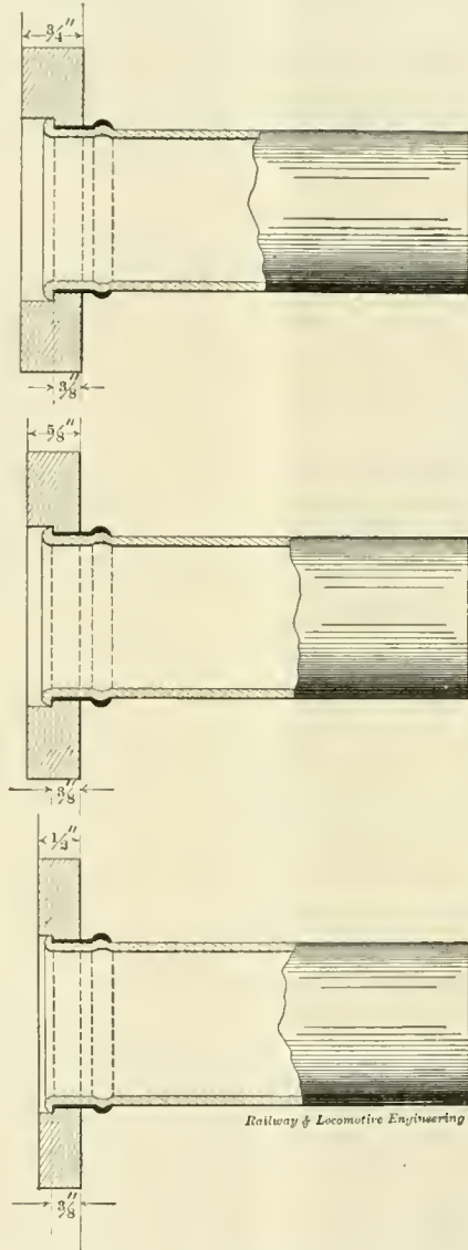
LAPE'S PATENT COUNTER-BORED FLUE SHEET.
